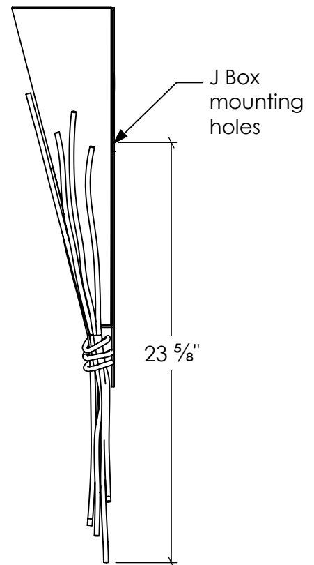
SIDE VIEW
