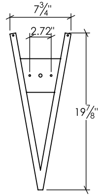
Backplate Mounting Detail Front View (Not to scale)
