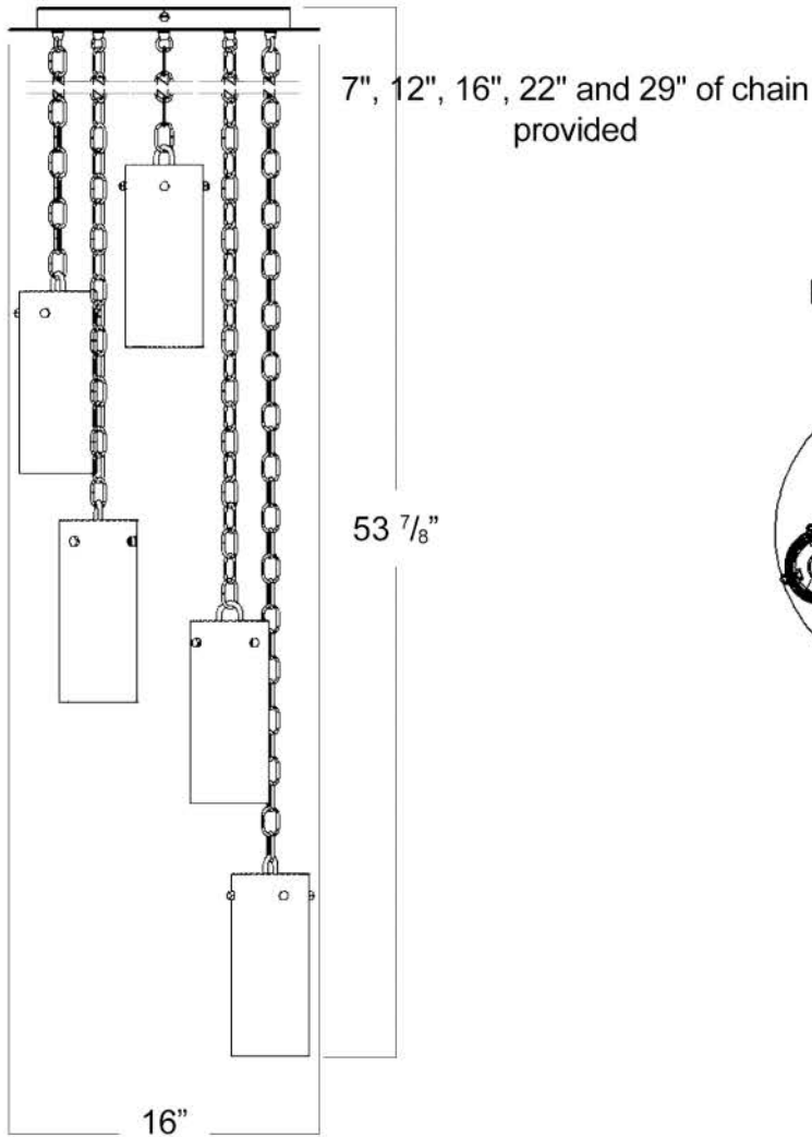
FRONT VIEW
