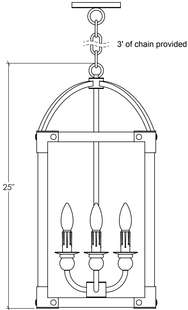
FRONT VIEW
