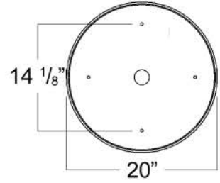
Canopy Mounting Detail
