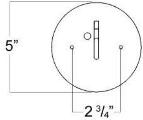
Canopy Mounting Detail
