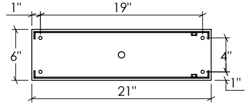
Backplate Mounting Detail Front View (Not to scale)
