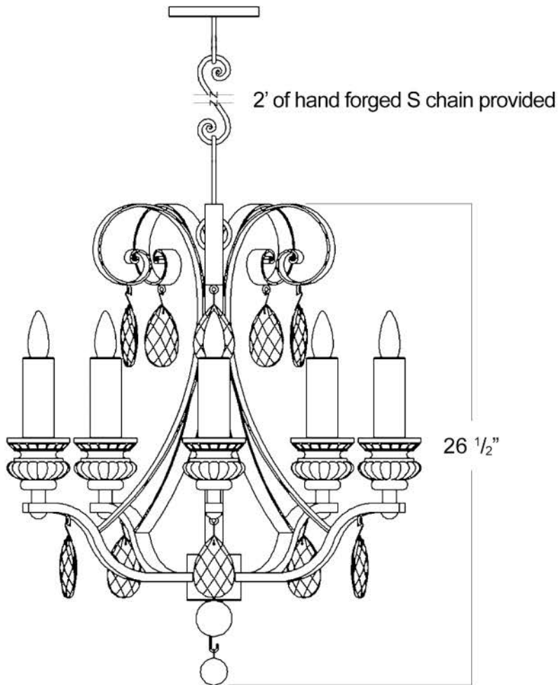
FRONT VIEW
